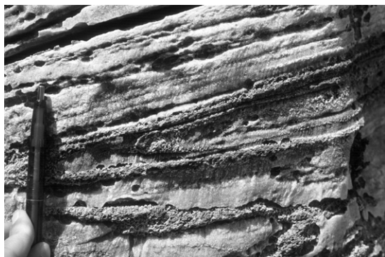
Fig. 3. Isoclinal fold in marble from NW Syros showing AP lineation at a large angle to the axial plane of the fold. Glaucophane lineation in the impure marble layers is parallel to the fold axes.
