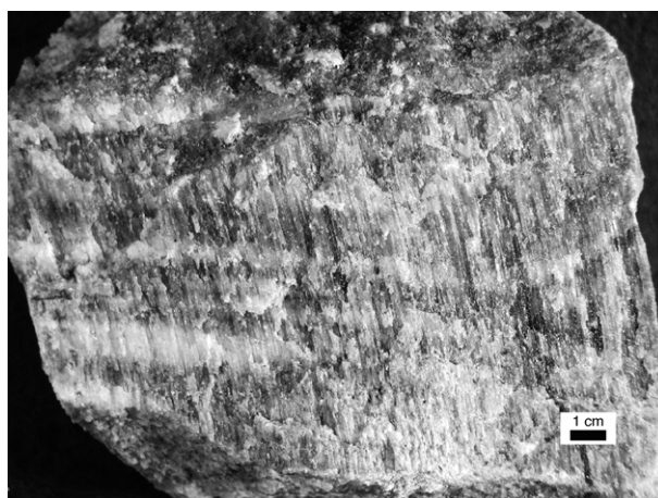
Fig. 2. Hand sample of marble from SE Syros (Katergaki) showing compositional banding and calcite pseudomorphs after aragonite. Foliation defined by phengite in adjacent layers is parallel to the compositional banding. Note the large angle between the compositional banding and the AP lineation.
