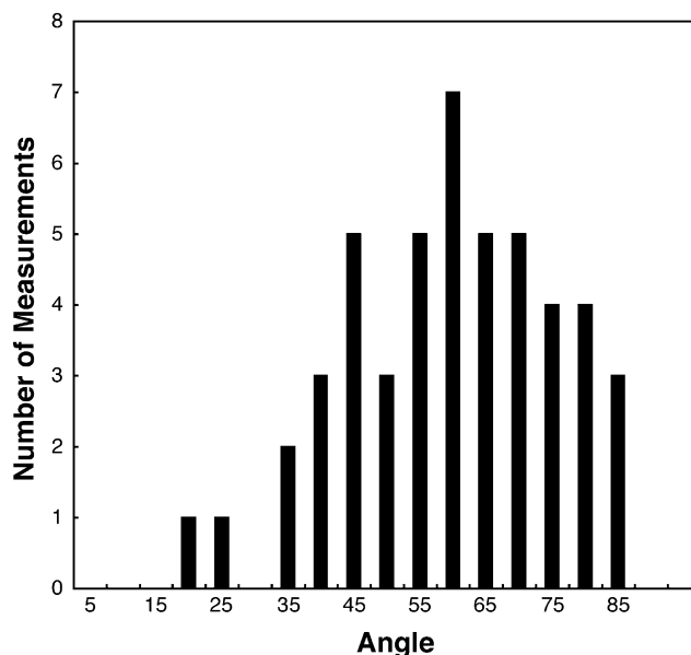
Fig. 5. Histogram of measured angles between AP lineation and foliation in marbles from Syros.
