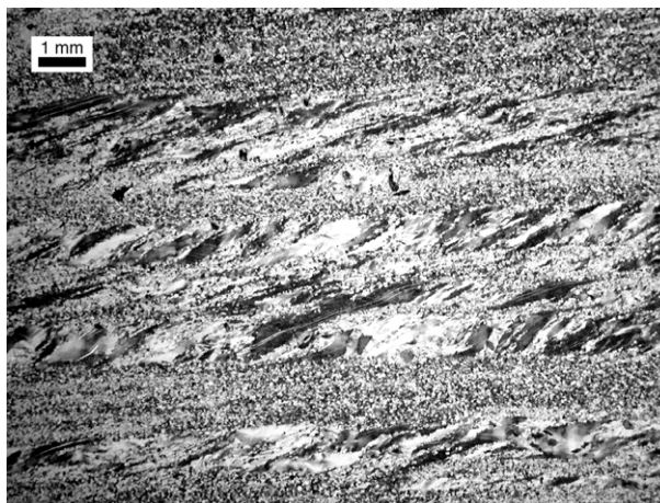
Fig. 6. Photomicrograph in crossed polarized light of a marble sample containing AP-bearing layers separated by fine-grained shear bands. The AP lineation is oriented at a low angle ( 22^\circ ) to the sheared layers.
